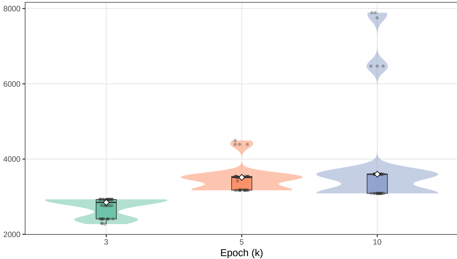
Generations until reaching minimum H
